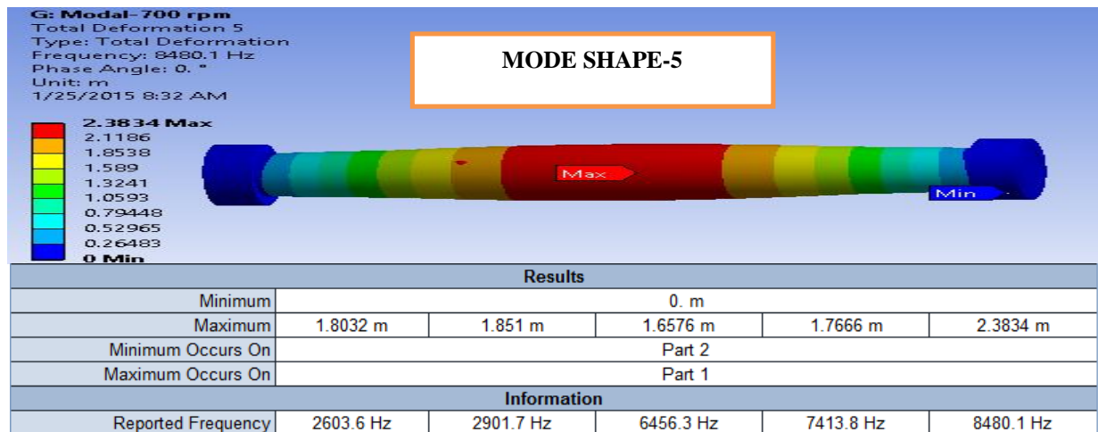
Fig 1: Mode shapes and frequency result by FEA without control mount
