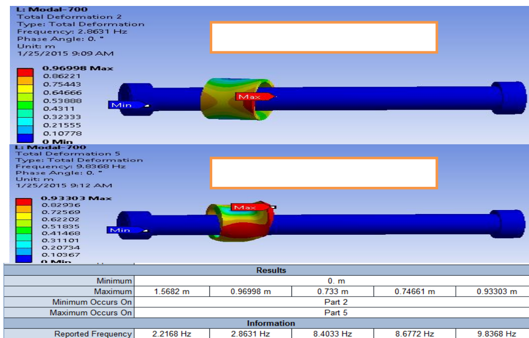
Fig.3 mode shapes result by FEA with control mount
