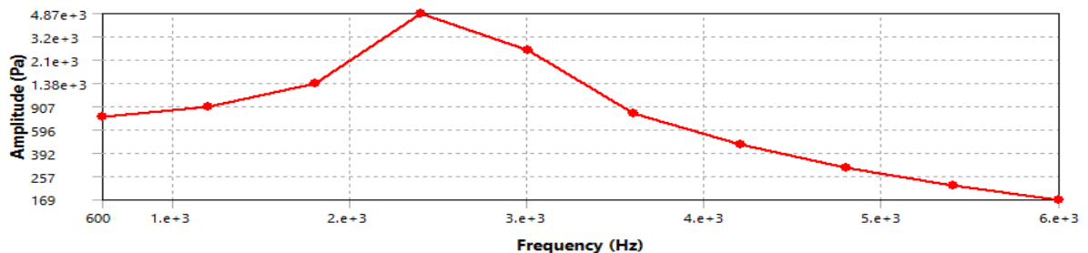
Fig 2. Frequency at harmonic response with load by FEA without control mount
