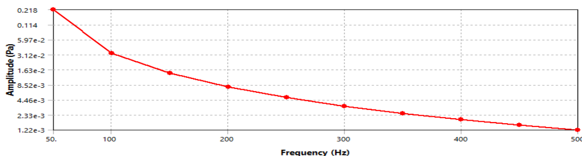
Fig 4. Frequency at harmonic response with load by FEA with control mount
